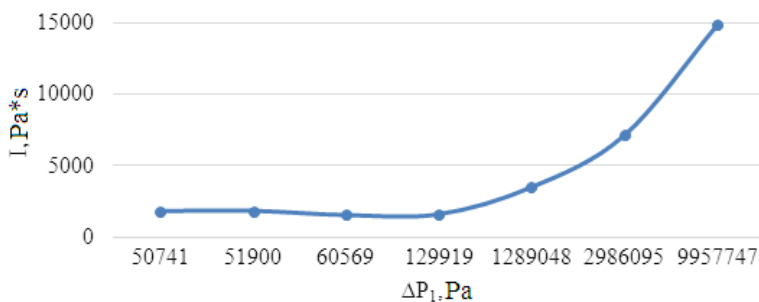
Fig. 2. Dependence of the impulse from the excess pressure in the explosion of charges of polymix GR4-T10 with different radii: a) at r_0 = 0.1 m; b) r_0 = 0.2 m
